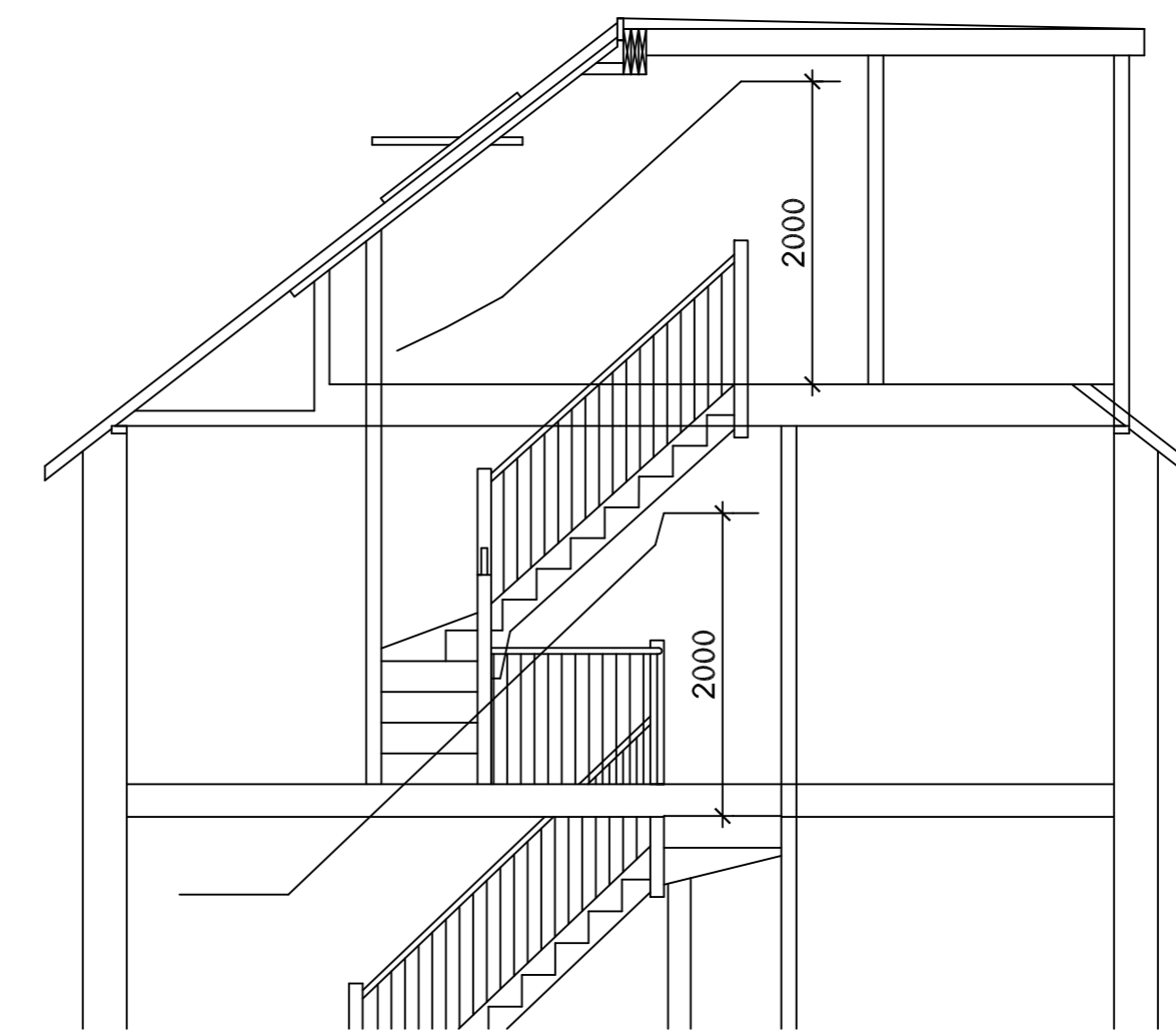
Proposed Section
